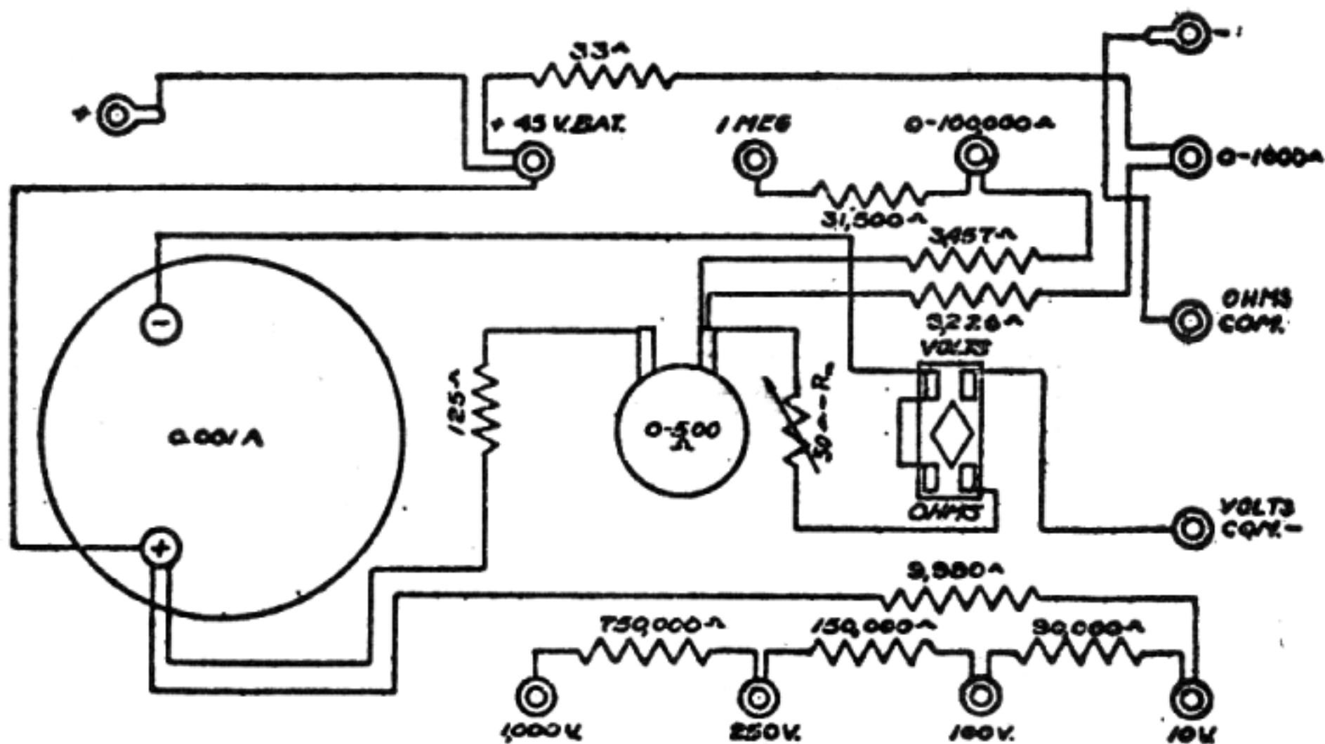
Model 44 Volt-Ohmmeter.
