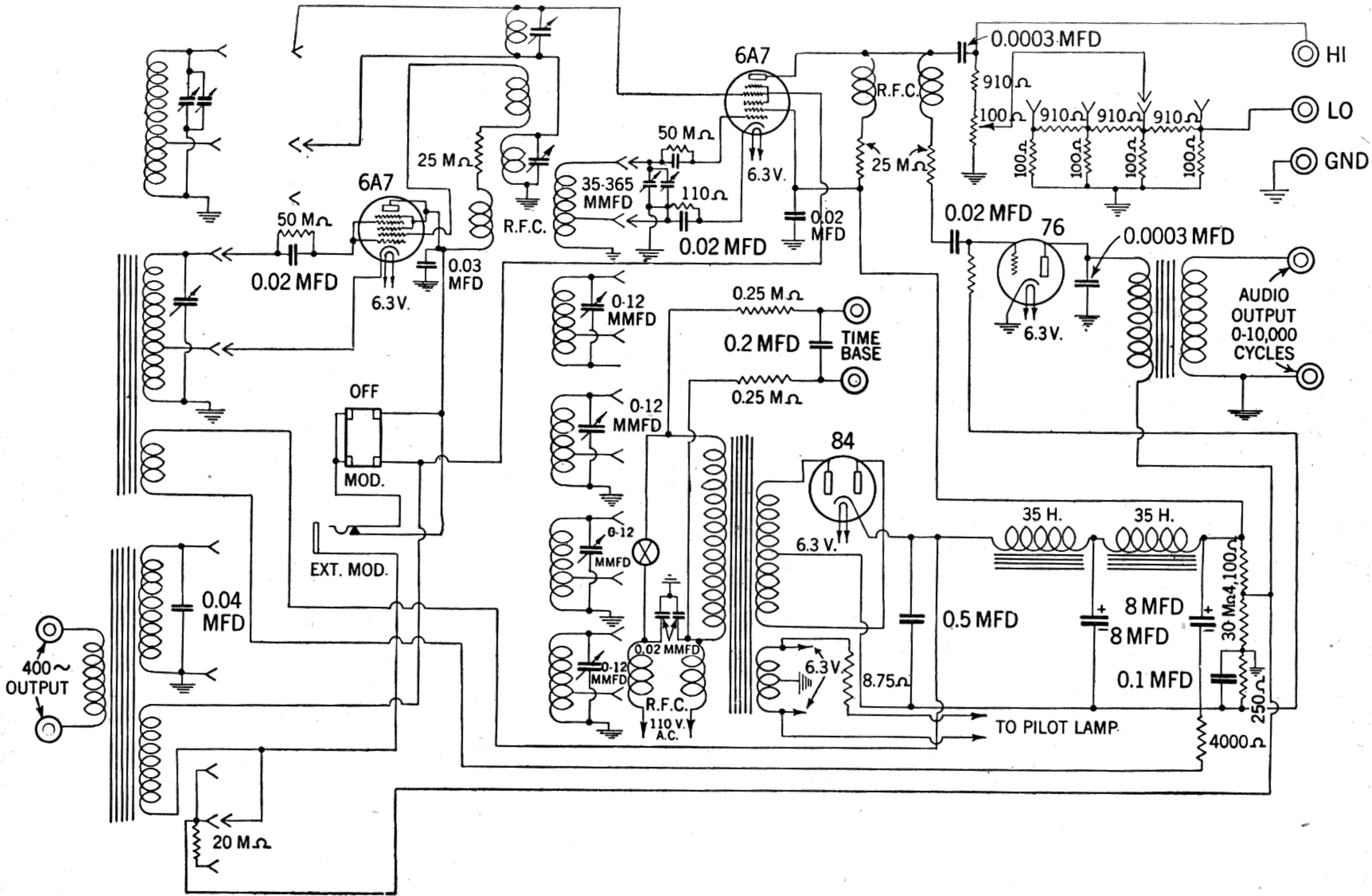
FIG. 29—Circuit diagram of Supreme Model 581 Signal generator.
