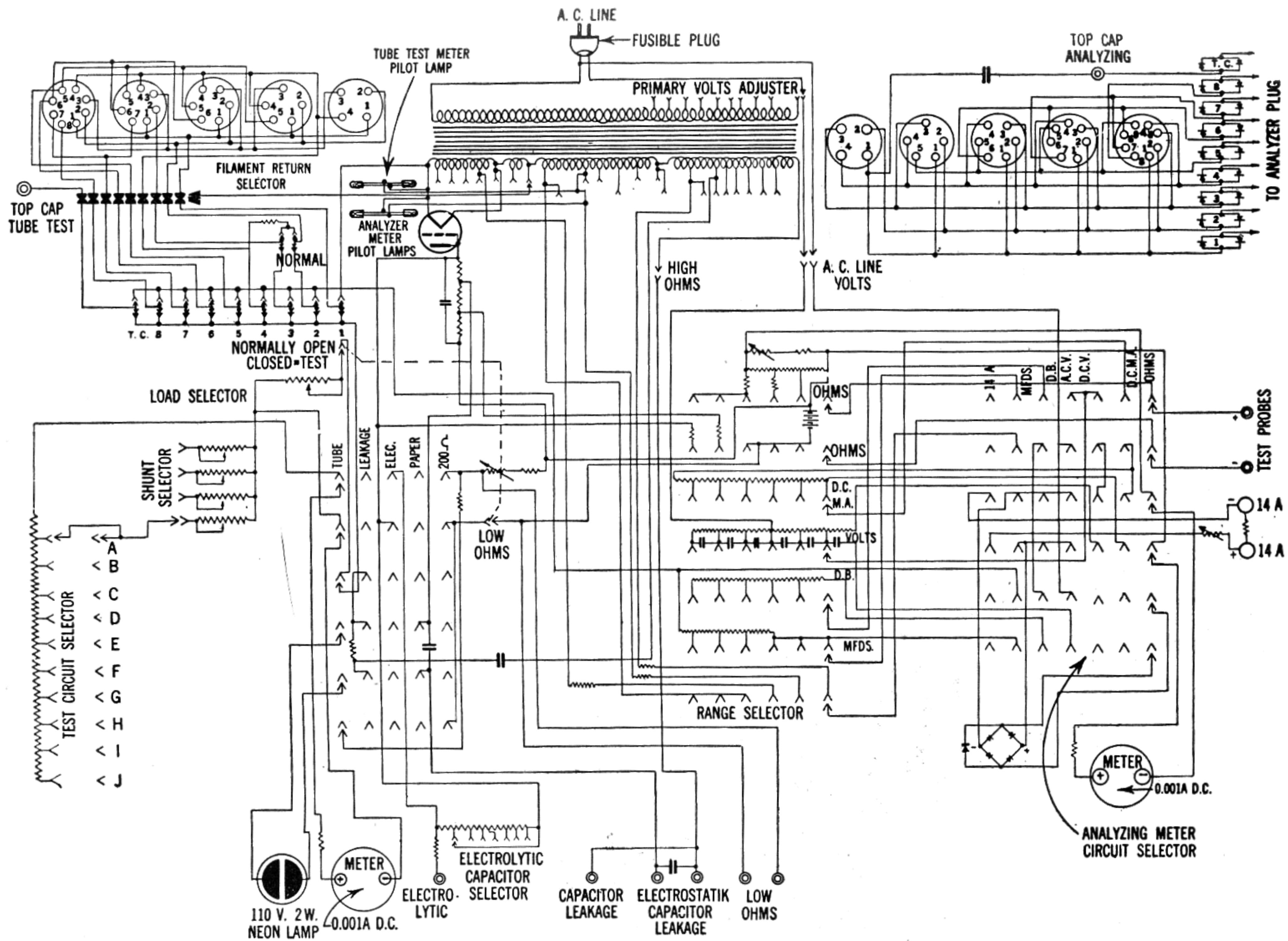
FIG. 23—Internal connection of Supreme Model 585 diagnometer.
