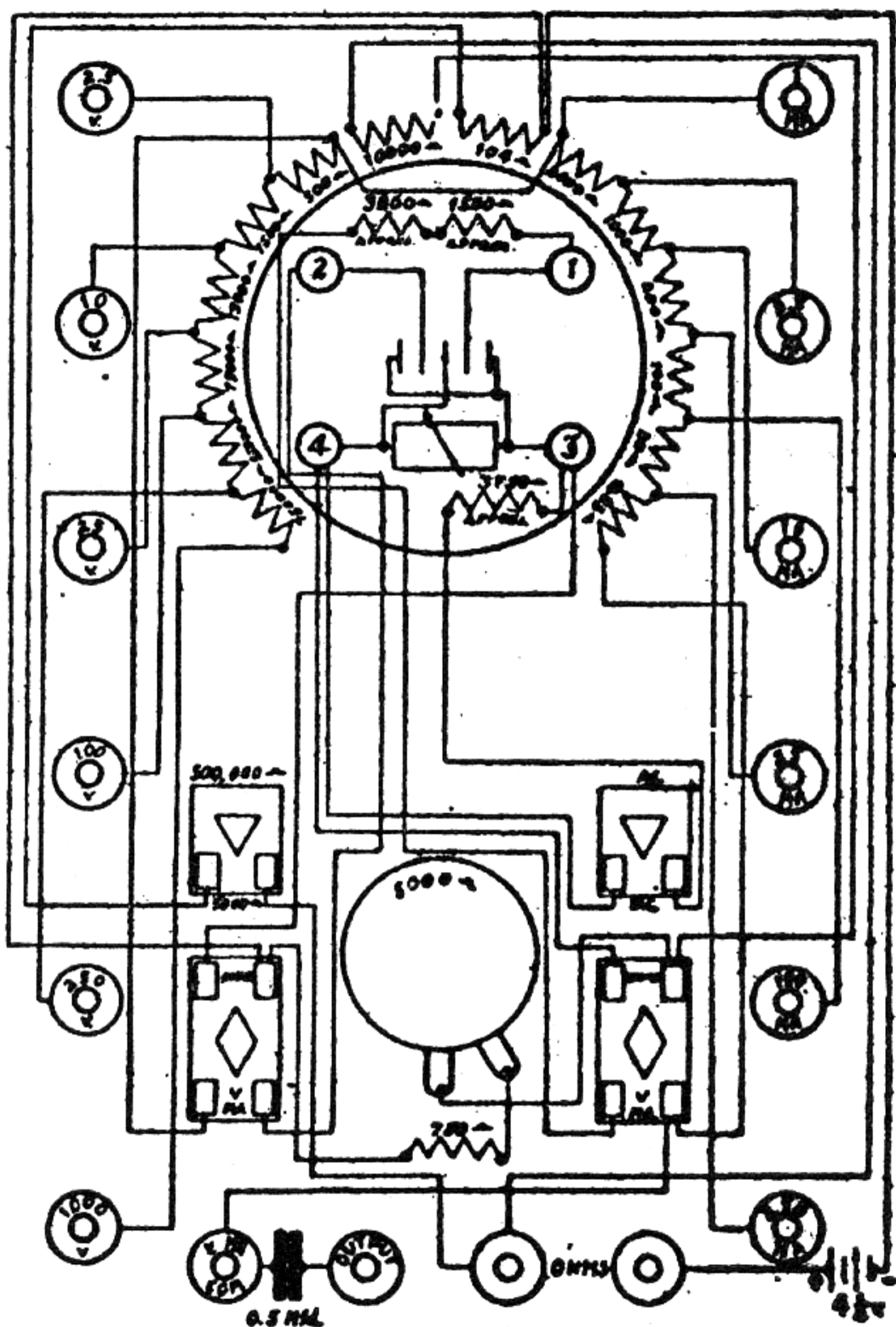
Model 75 AC-DC Volt-Ohm Milliammeter
