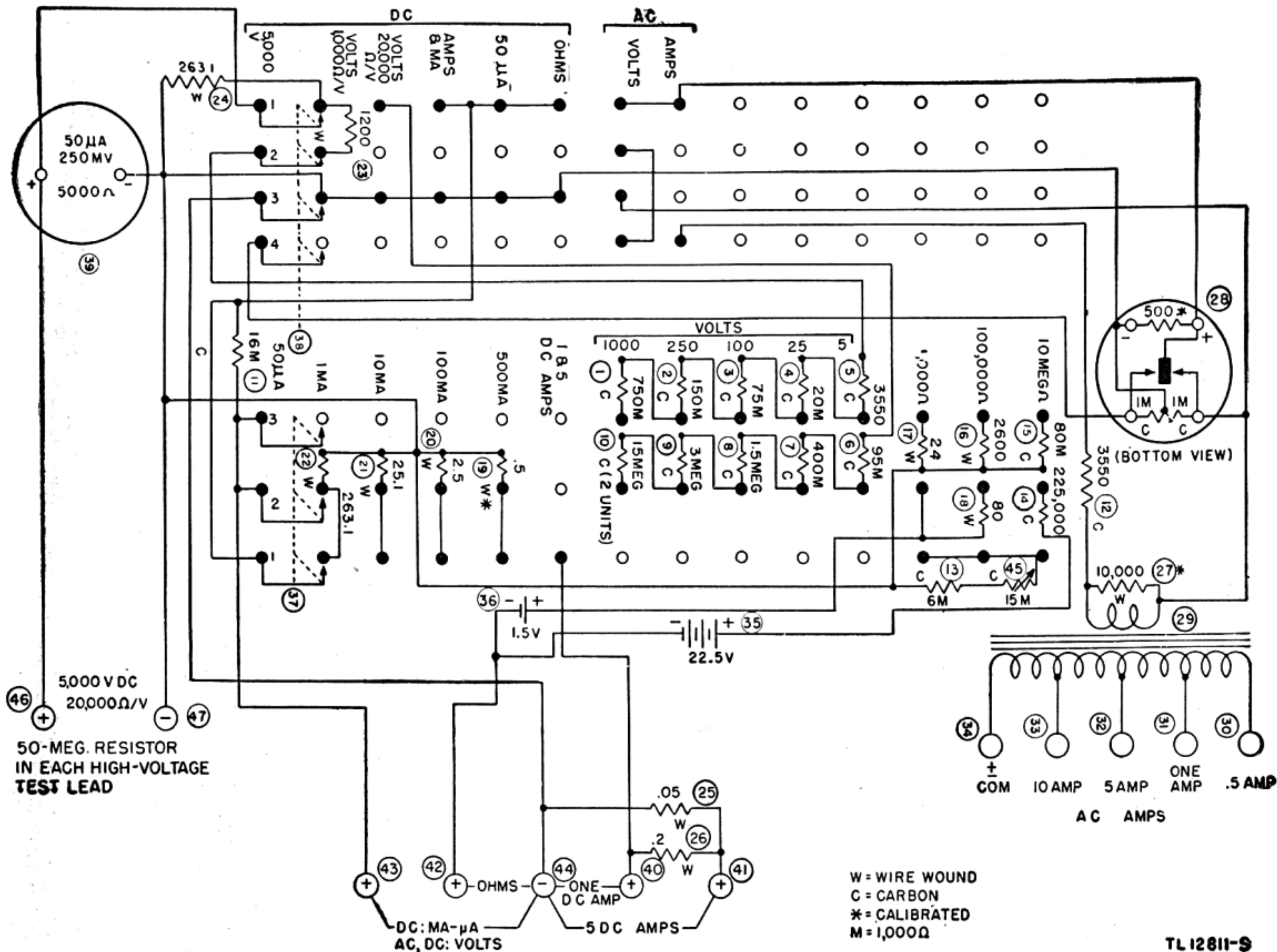
Test Unit I-176, schematic diagram.
